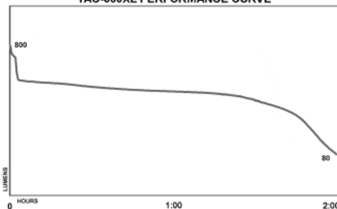
TAC-560XL PERFORMANCE CURVE
